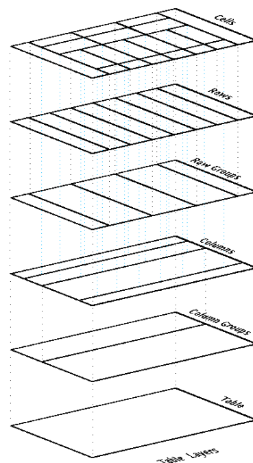
Figure 21 Table Structure
