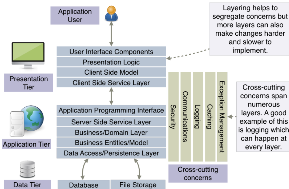
Figure 1.2 A typical three-tier application is usually made up of presentation, application, and data tiers. A tier may have multiple layers with specific responsibilities. A developer can choose how layers will interact with each other. This can be strictly top-down or in a loose way, where layers can bypass their immediate neighbors to talk to other layers.
