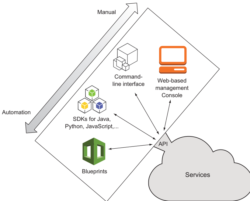
Figure 1.12 Tools to interact with the AWS API
