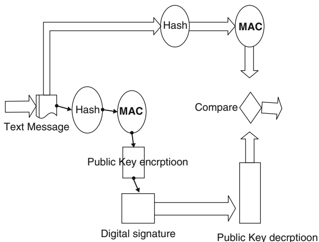
Fig. 11.9 Verifying a digital signature in message authentication
