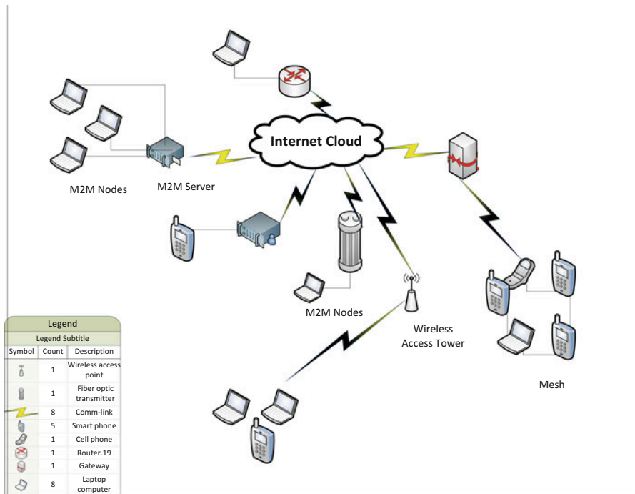
Fig. 24.3 IoT communication network architecture
