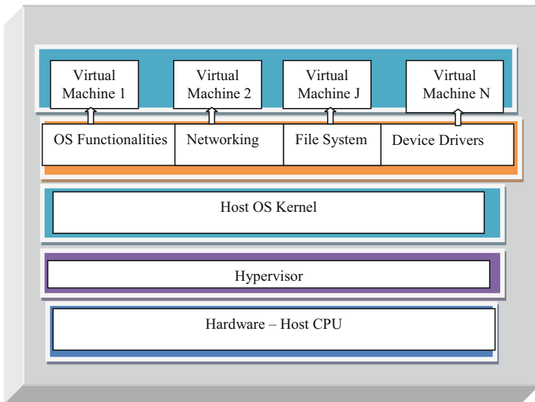
Fig. 22.2 Type-1 hypervisor
