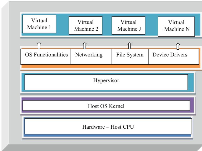
Fig. 22.3 Type-2 hypervisor
