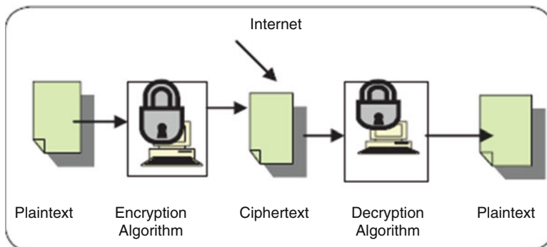
Fig. 11.1 Symmetric encryption
