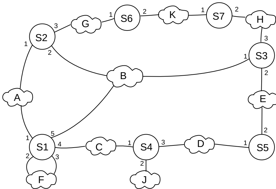
Fig. 15:: Switched Ethernet with potentially multiple hosts connected to switch ports
