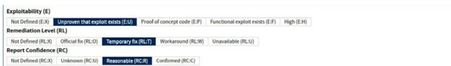
Figure 21-3. The CSRF temporal score scores a vulnerability based on the maturity of security mechanisms in your codebase
